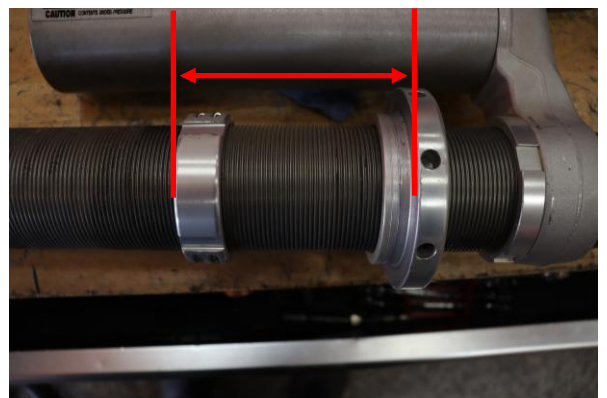
Step 16. Install the Eibach crossover ring and set to 100mm (3 15/16in.) from bottom of spring seat to bottom of crossover ring.
