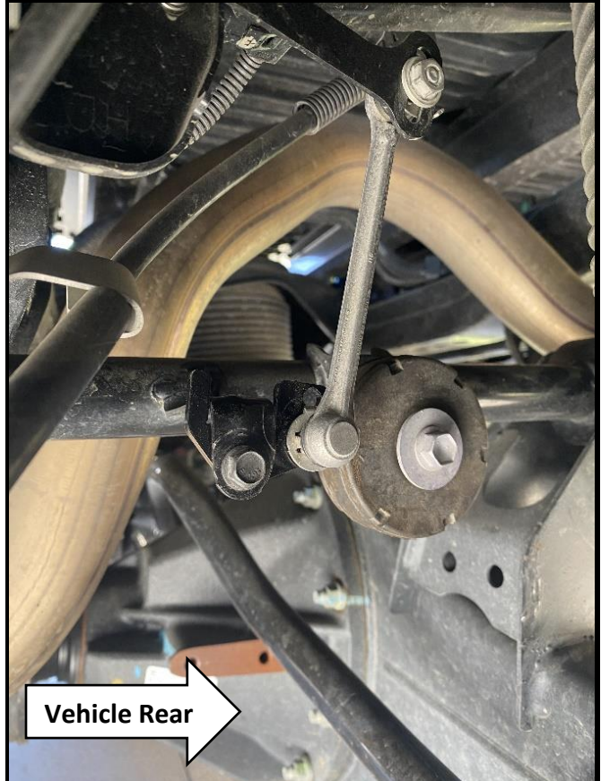
Figure 2: Install 3061 Ride Height Sensor Bracket. Driver side shown.
