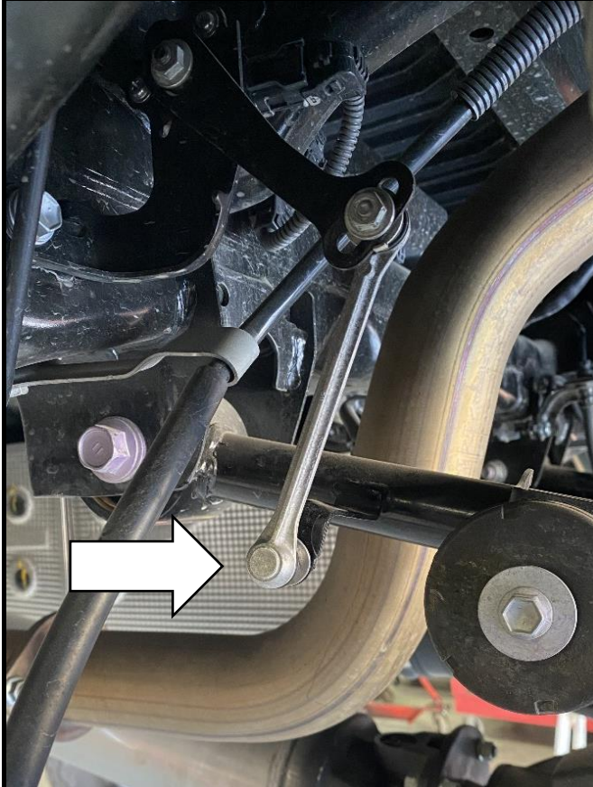
Figure 1: Remove ride height sensor linkage from upper control arm. Driver side shown.
