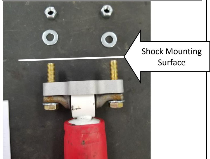
Figure 6: Install Spacer and Hardware
