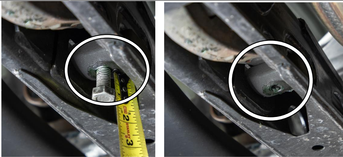
Figure 1: Measure and Remove Torsion Bar Adjuster Screw
