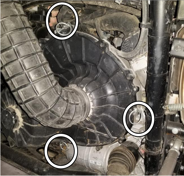
Figure 1: Installed Pro XP Clutch Cover with Pins (Rear Pins)
