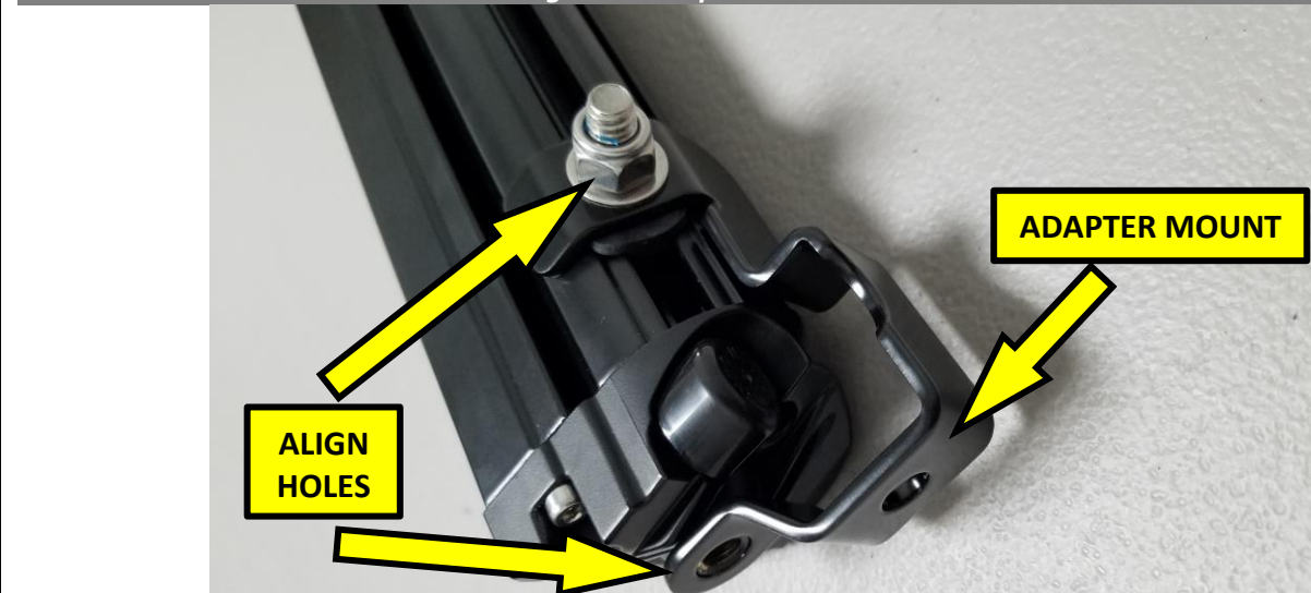
Figure 3: Adapter Mount Installation
