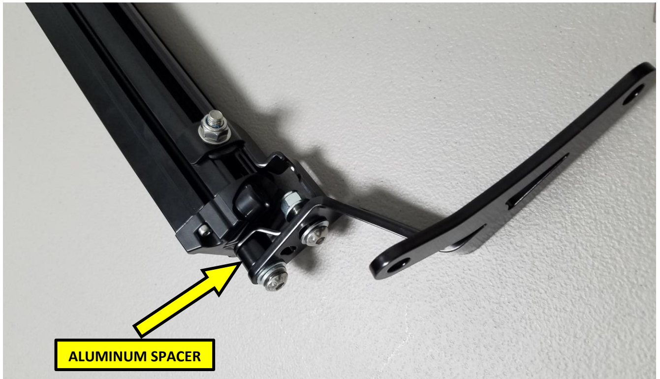
Figure 5: Front Mount Installation
