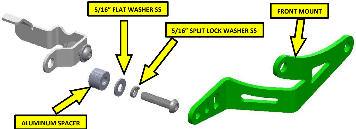
Figure 4: Front Mount
