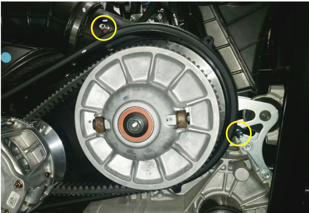
Figure 1: XP1k Clutch Cover Rear Two Pin Locations
