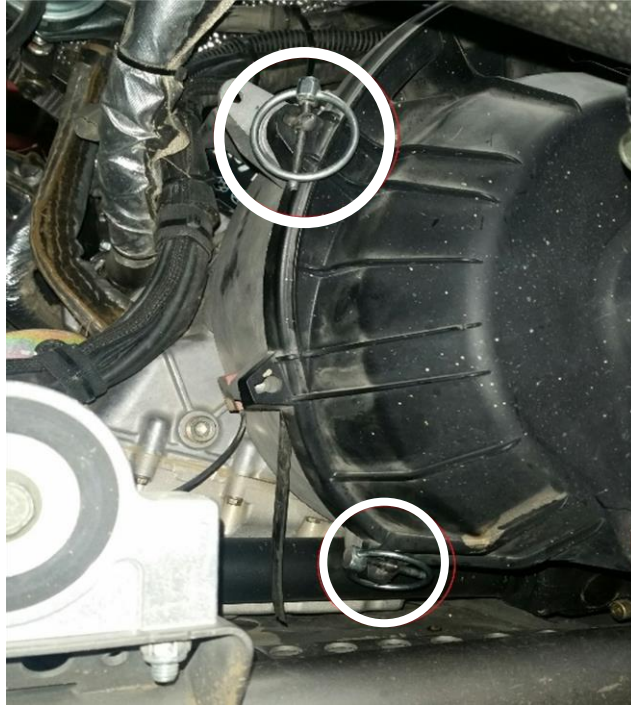
Figure 2: Installed XP Turbo Clutch Cover with Pins (Front Pins)
