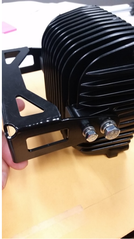
Figure 5: bolt bracket onto light using bolts from the bracket kit and washers from the light kit.
