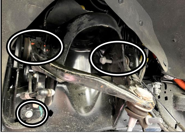
Figure 11: UCA Pivot Bolts and Sensor Bolt Removal
