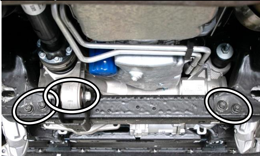
Figure 13: OEM Rear Crossmember Attachment Points.
