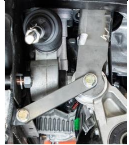
Figure 38: Differential Mount Brace Installed.
