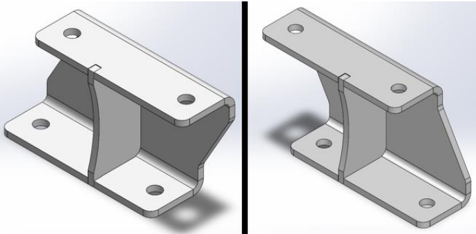
Figure 51: Weldments 8640 & 8641.
