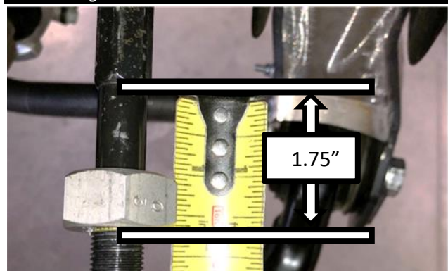
Figure 24: Mark & Cut OEM Inner Tie Rod.
