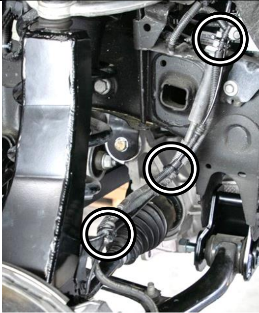
Figure 61: Line & Wire Routing.
