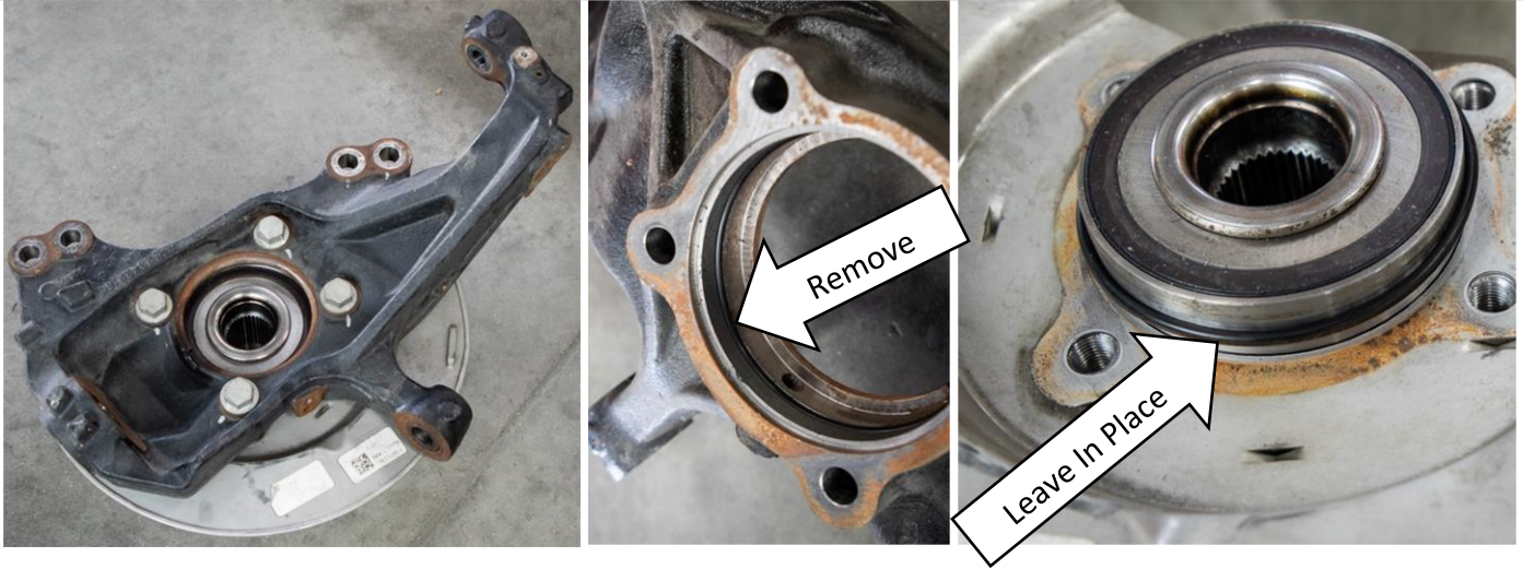
Figure 41: Disassemble Hub Assembly
