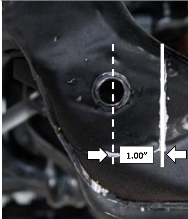
Figure 26: Mount Differential Drop Bracket Driver Side
