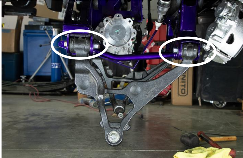
Figure 68: Lower Control Arm Bolts that do NOT get torqued at this step
