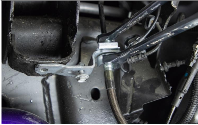
Figure 29: Cognito Extended Stainless-Steel Brake Lines
