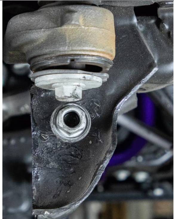
Figure 27: Cut Mount Differential Drop Bracket Passenger Side
