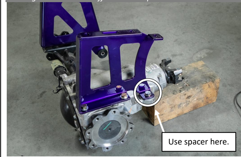
Figure 31: Mount Differential Drop Bracket Driver Side
