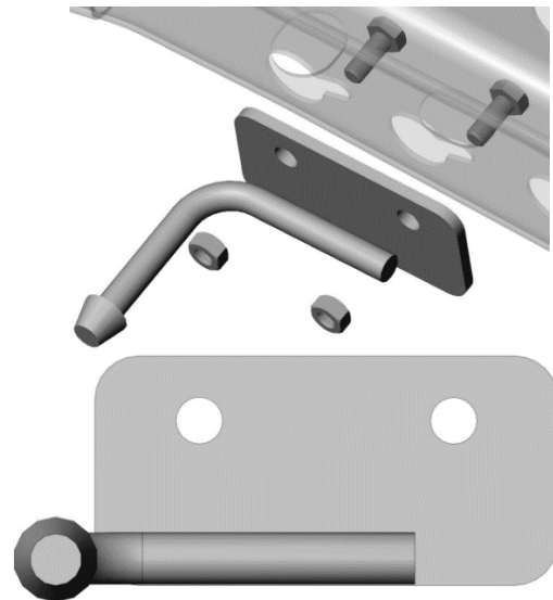
Image 2 NOTE: 2.3L Requires Hanger Bracket (05-245239) Included. See Step 8
