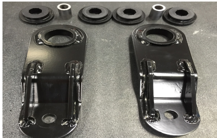
Figure 11: Traction Bar Shackle Parts
