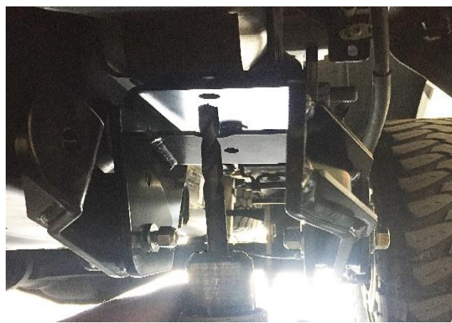
Figure 6: Frame Mount Hole Locations
