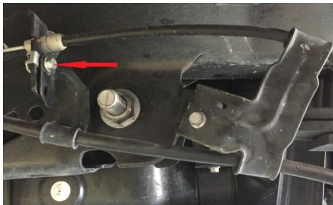
Figure 2: Brake Cable Bracket Mounting Bolt
