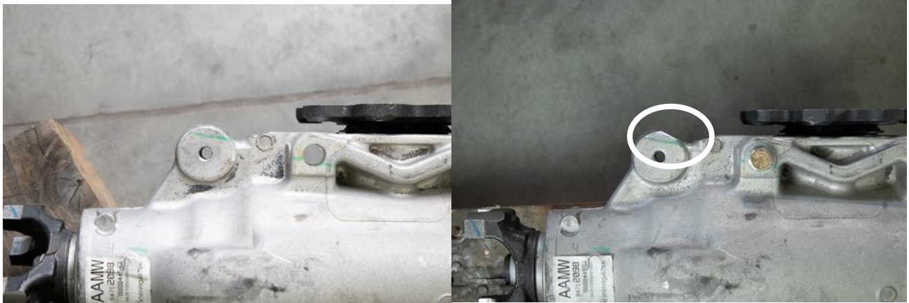
Figure 25: Notch on Differential
