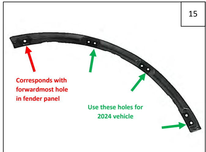
Holes to be used to install Inner Bracket for 2024 vehicle (rearwardmost of each pair of holes).
