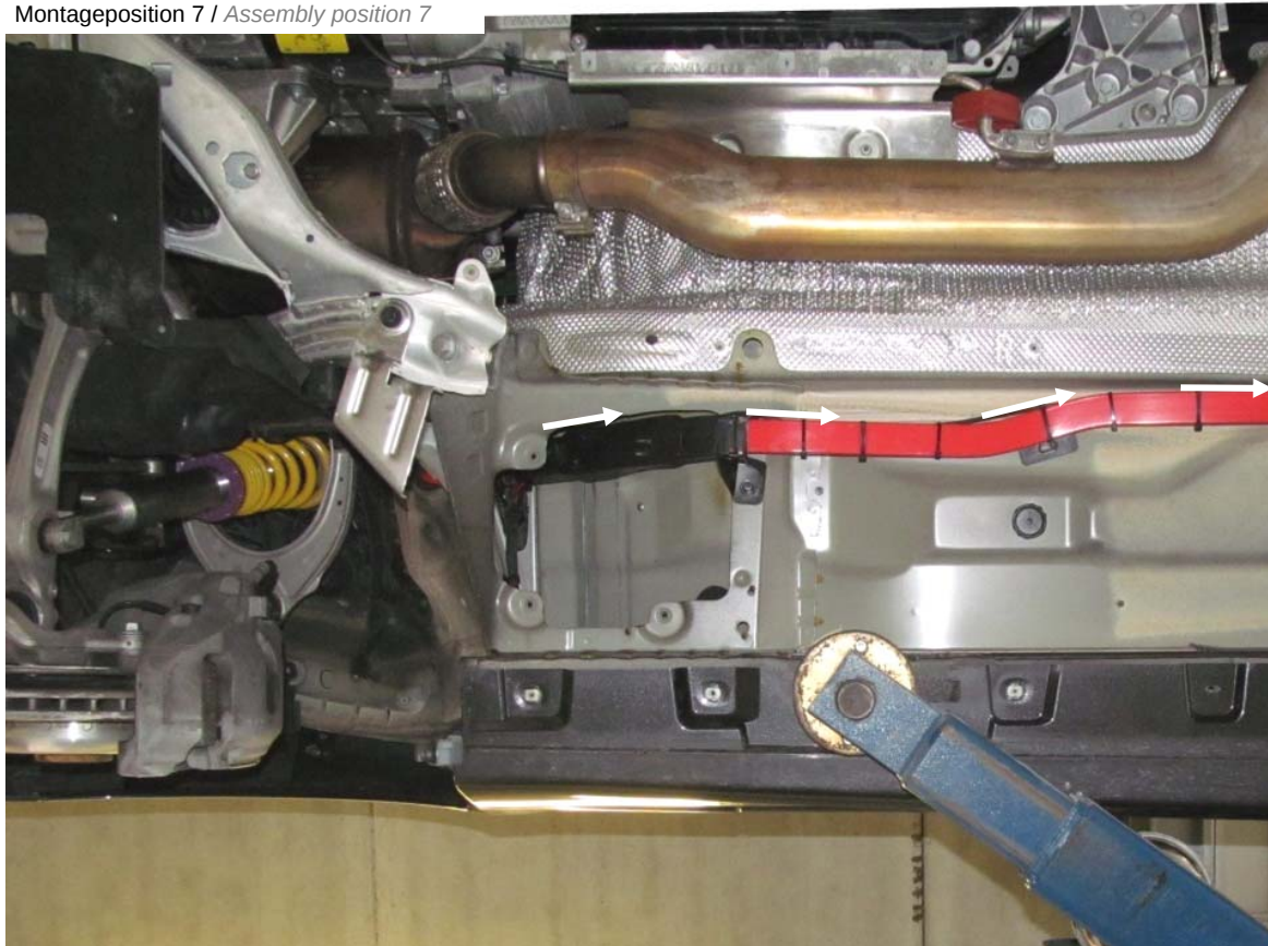
Montageposition 7 / Assembly position 7
