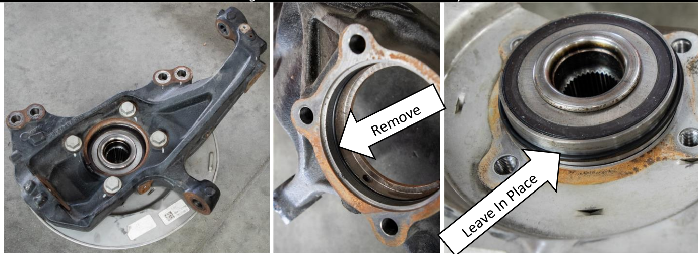
Figure 48: Disassemble Hub Assembly
