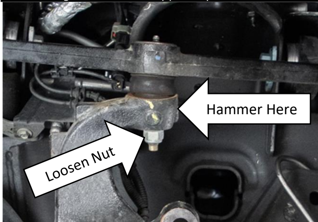
Figure 14: Brake Upper Tapered Seat
