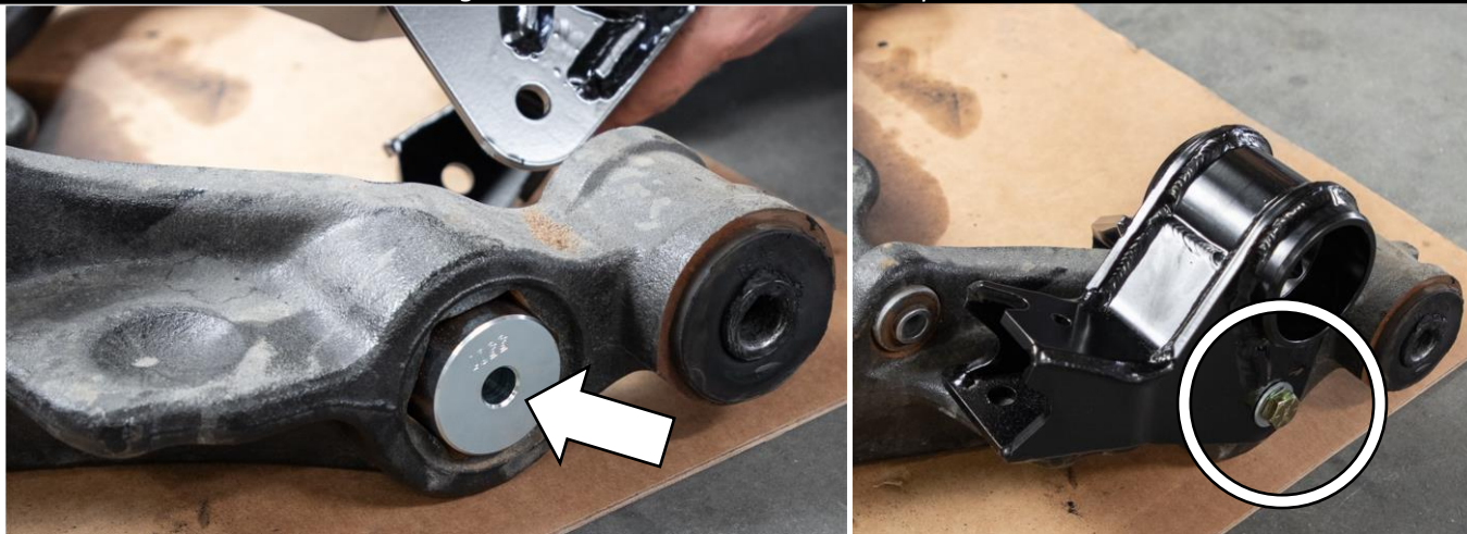
Figure 42: Install Non Torsion Bar Drop Bracket
