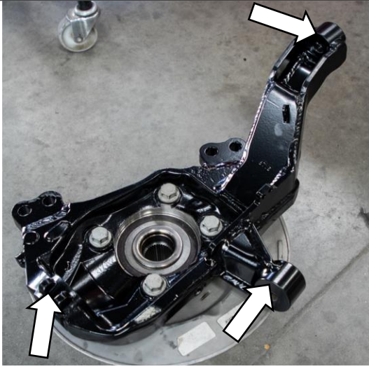
Figure 52: Prepare Spindle
