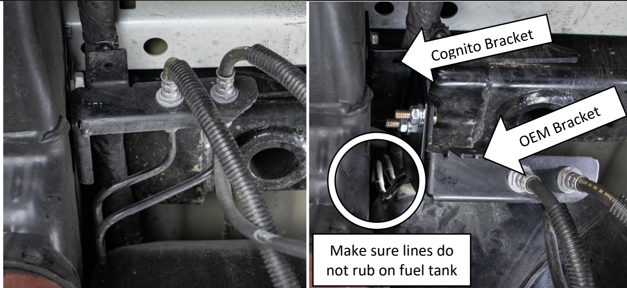
Figure 58: Install Cognito Rear Brake Line Brackets
