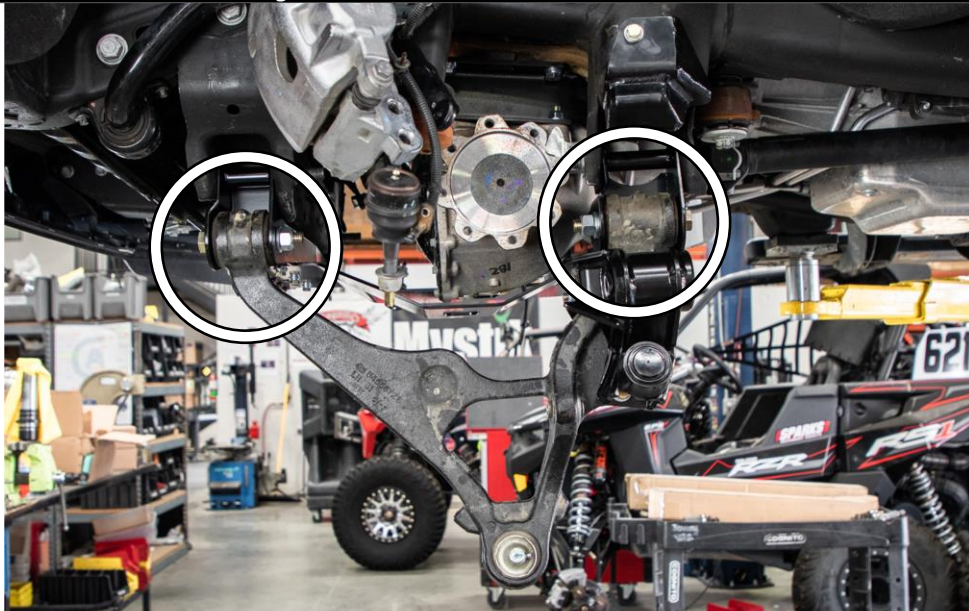
Figure 45: Reinstall Lower Control Arms
