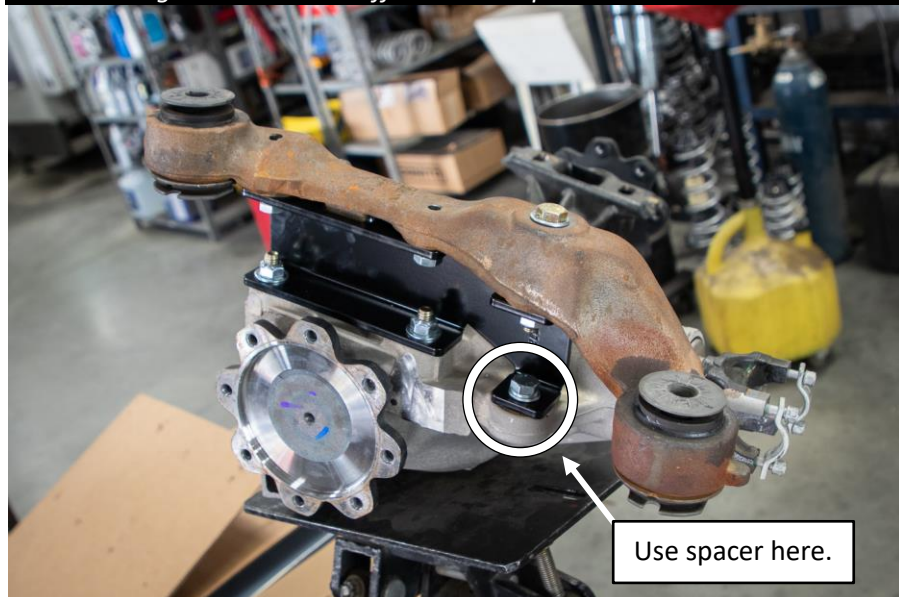
Figure 28: Mount Differential Drop Bracket Driver Side
