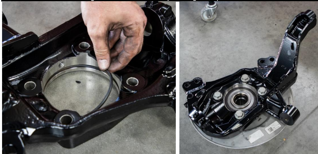
Figure 49: Hub Assembly on Cognito Spindle
